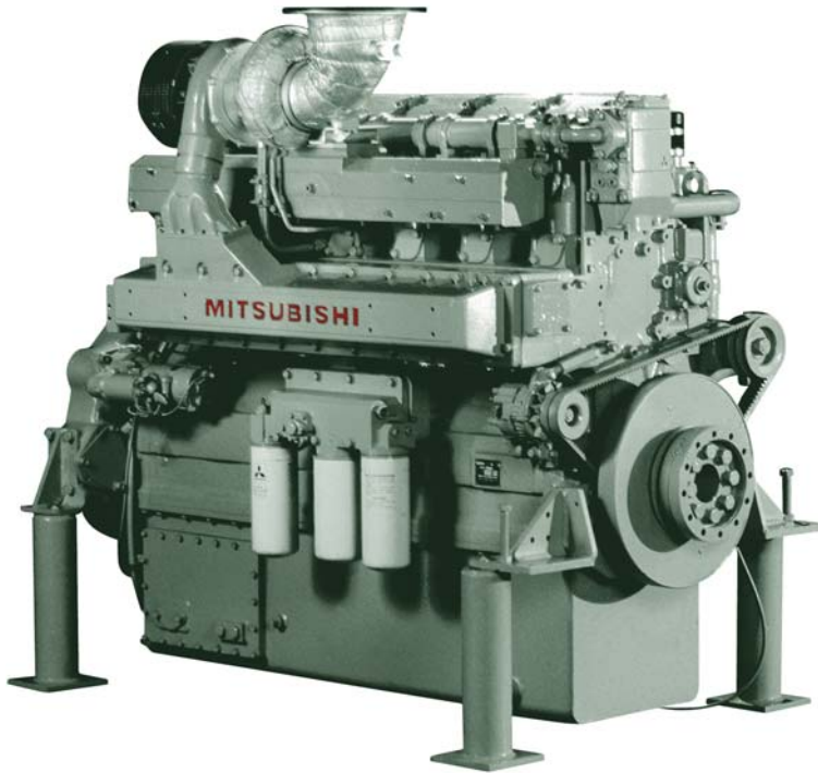
Emergency / Harbour Generator: Mitsubishi S6R-MPTA, 595kW / 1,800rpm
